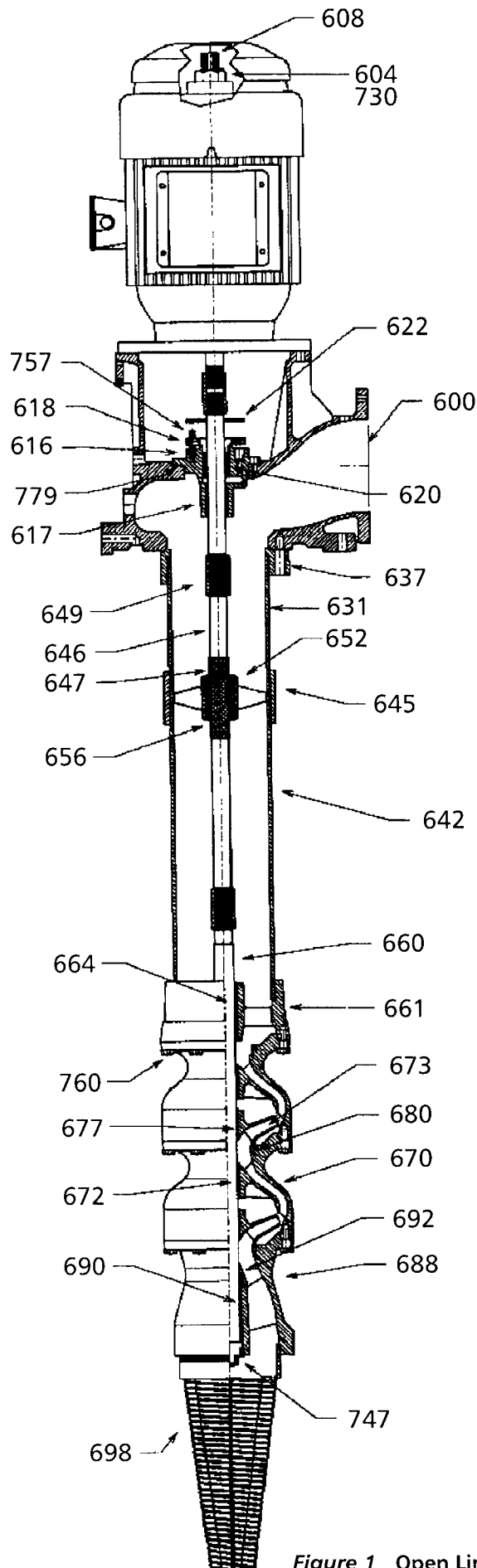
Figure 1 Open Lineshaft Pump
